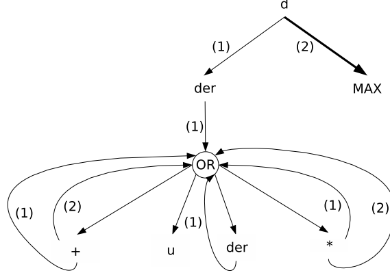
Fig. 1. Rigid type graph for Example 7
