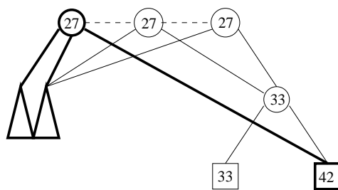
Fig. 6: Insertion of key 33 into a transcript tree.
