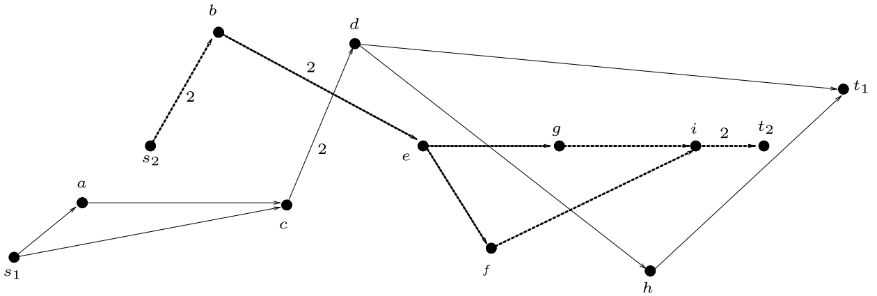
Fig. 5. A feasible solution to the flow problem where x (resp. y ) follows the full (resp. dotted) arcs.
