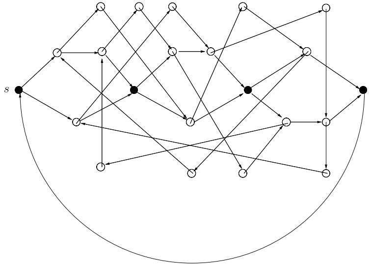
Fig. 1. An illustration of the digraph D_{\mathcal{F}} when \mathcal{F} = (x_1 + \bar{x}_2 + x_3)(x_1 + x_2 + \bar{x}_3)(\bar{x}_1 + x_2 + \bar{x}_3) . The black vertices are the vertices u_i, v_i of the variable gadgets.
