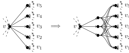
Fig. 4. Constructing R_8(\mathcal{F}) from R_6(\mathcal{F}) .
