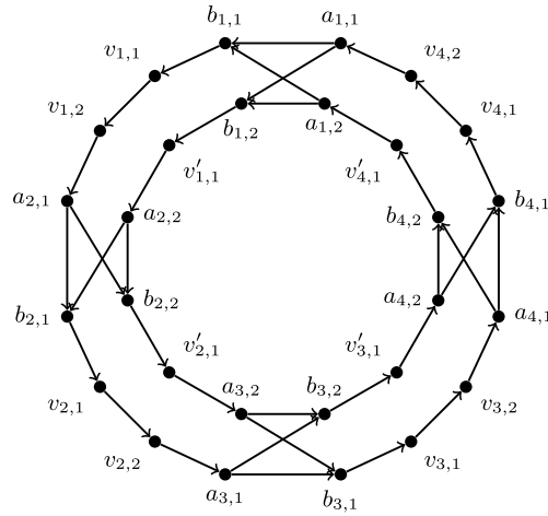
Fig. 1. A ring digraph.
