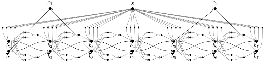
Fig. 3. The digraph D(\mathcal{F}) when \mathcal{F} has the clauses C_1 = \bar{x}_1 \vee x_2 \vee \bar{x}_3 and C_2 = \bar{x}_5 \vee x_6 \vee \bar{x}_7 .
