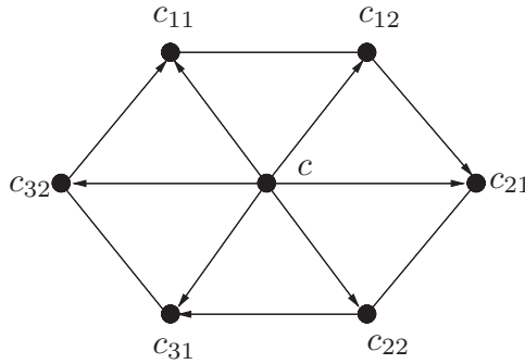
FIGURE 2 A partially oriented wheel W
