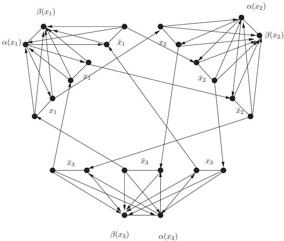
FIGURE 3 Part of the digraph H'(\mathcal{F}) when \mathcal{F} = (x_1 \vee x_2 \vee \bar{x}_3) \wedge (\bar{x}_1 \vee \bar{x}_2 \vee x_3) \wedge (x_1 \vee \bar{x}_2 \vee \bar{x}_3) . For better readability the vertices c_1, c_2, c_3 are not shown.
