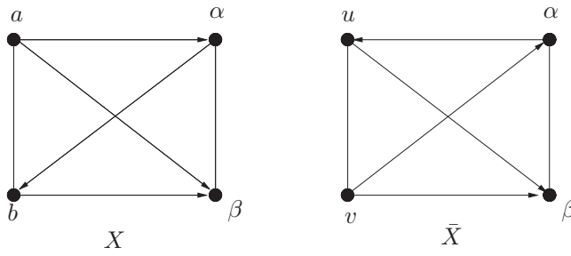
FIGURE 1 Two different labelings of the same partially oriented complete graph on four vertices. For later convenience we name these X, \bar{X} .
