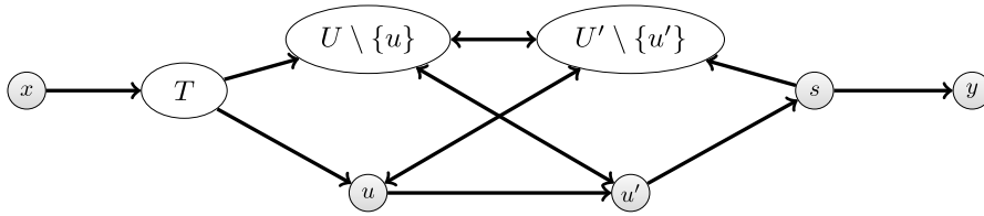
Fig. 1. An (x, y) - (i, p) -connector, where |T| = i and |U \setminus \{u\}| = p - 1 and |U' \setminus \{u'\}| = p - 1 .
