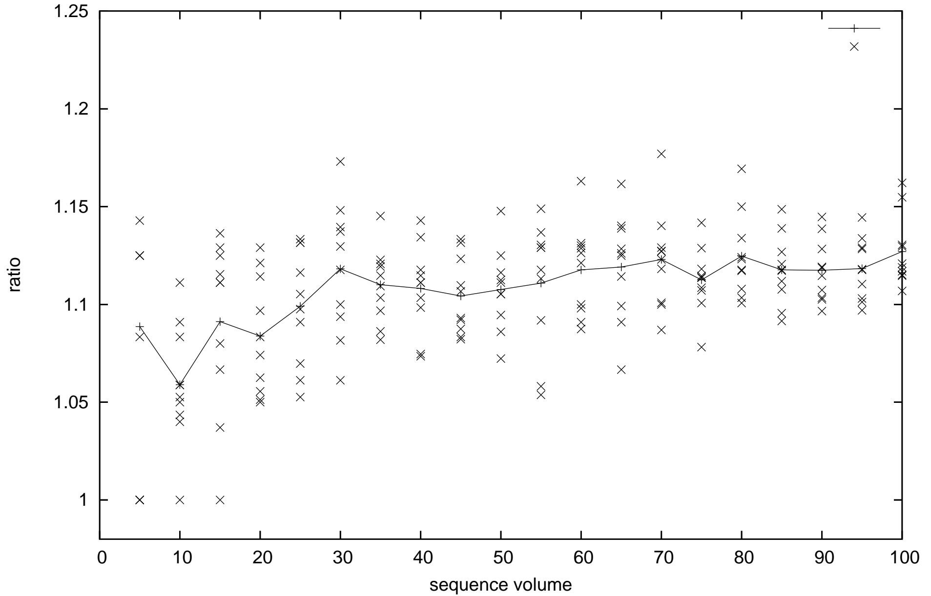
Dual Bin Packing, uniform data, comparing FirstFit to WorstFit, sample size 10
