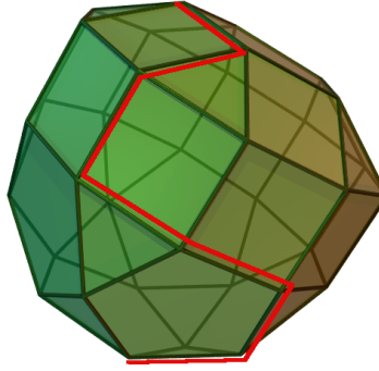
Figure 2.12: . The shortest path between any two vertices of a polyhedron may contain an exponentially growing number of vertices as the dimension grows.
