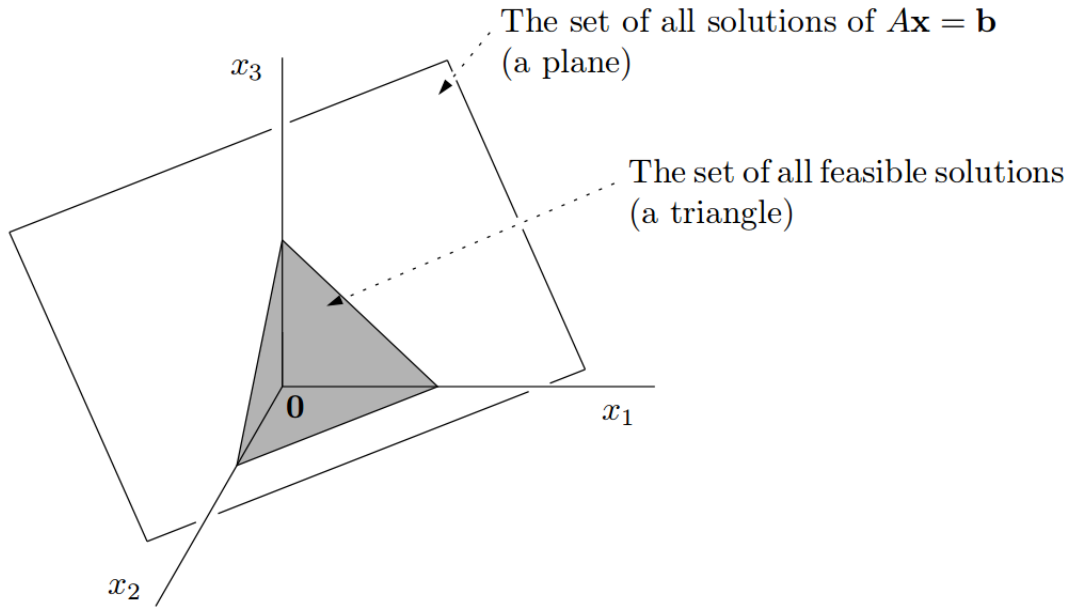
Figure 2.4: The intersection between A\mathbf{x} = \mathbf{b} and \mathbf{x} \geq \mathbf{0} in \mathbb{R}^3 .
