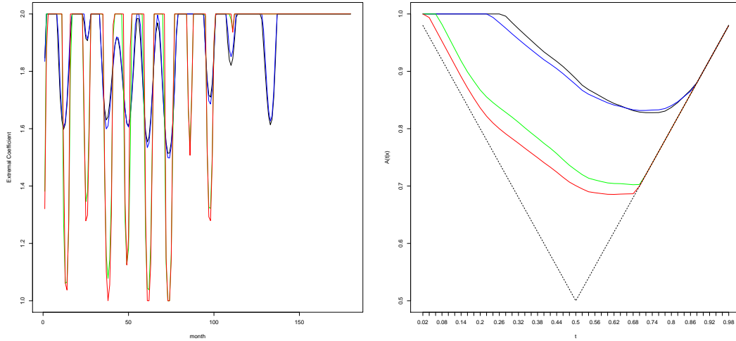
FIG 2. Air pollution data: time plot of the estimate for the conditional extremal coefficient (left) and estimate for the conditional Pickands dependence function in April 2002 (right), \alpha = 0 (black), \alpha = 0.1 (blue), \alpha = 0.5 (green) and \alpha = 1 (red).
